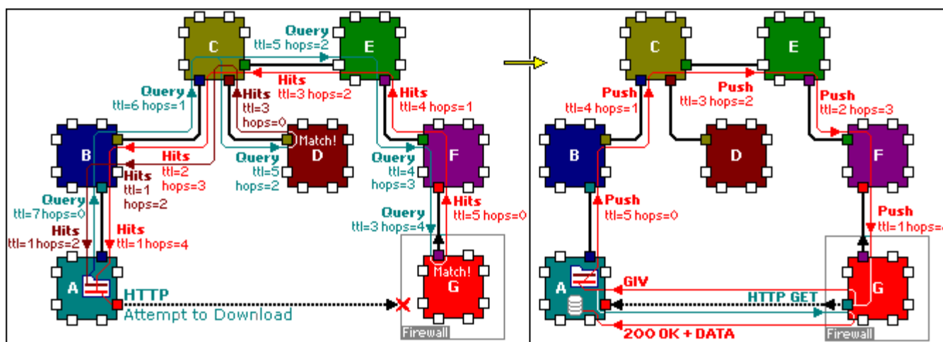
Example 2. Query/QueryHit/Push routing
